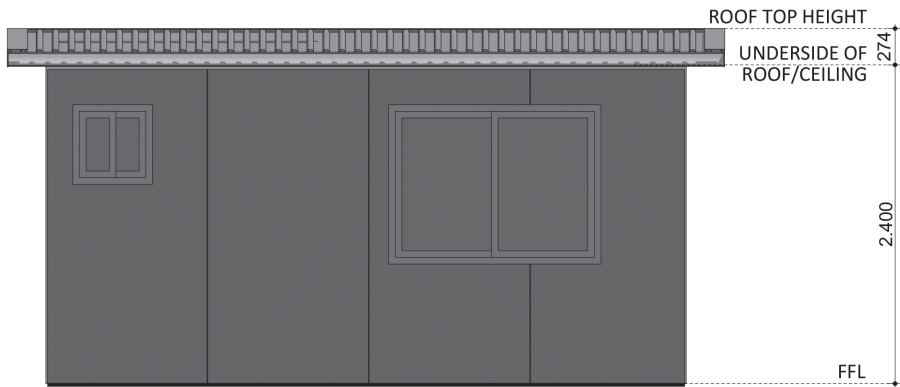
ELEVATION 03
