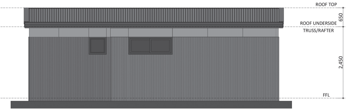
ELEVATION 03
