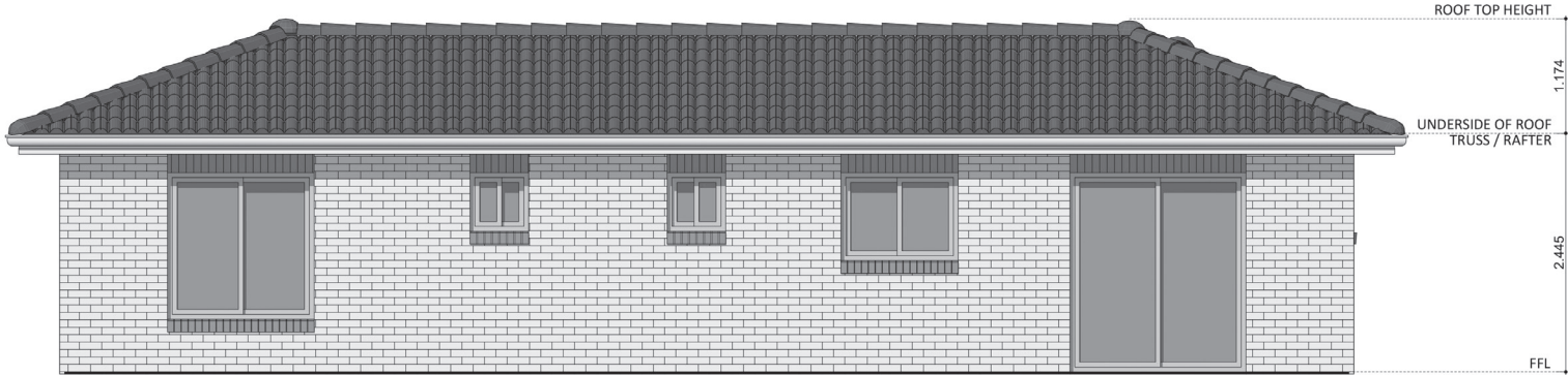
ELEVATION 03
