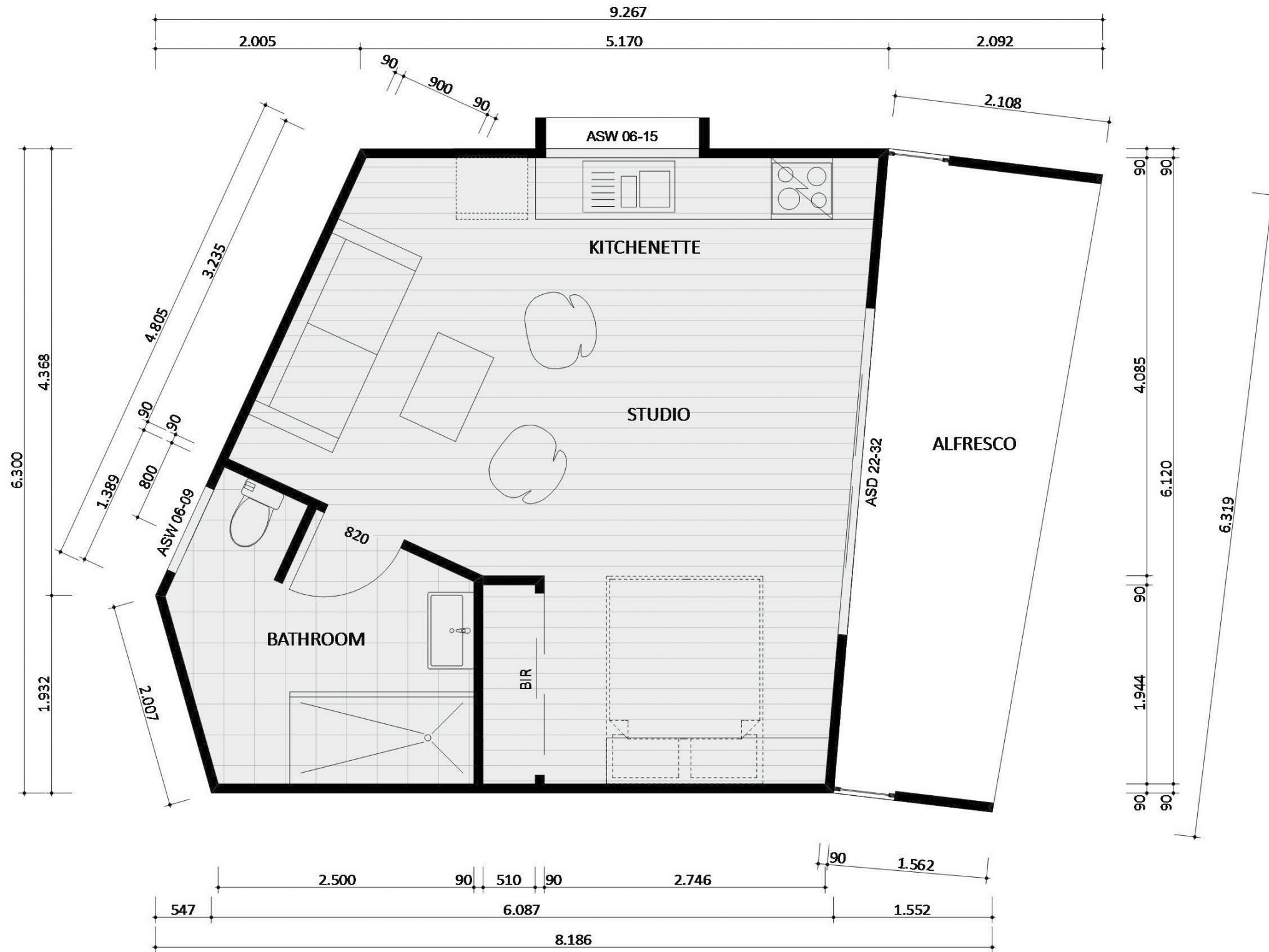
FLOORPLAN DIMENSION DESIGN 90
