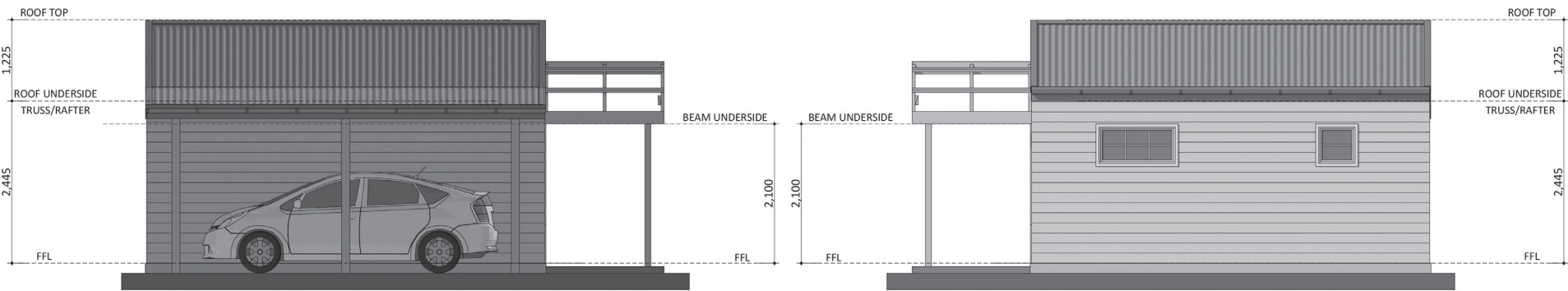
ELEVATION 03
