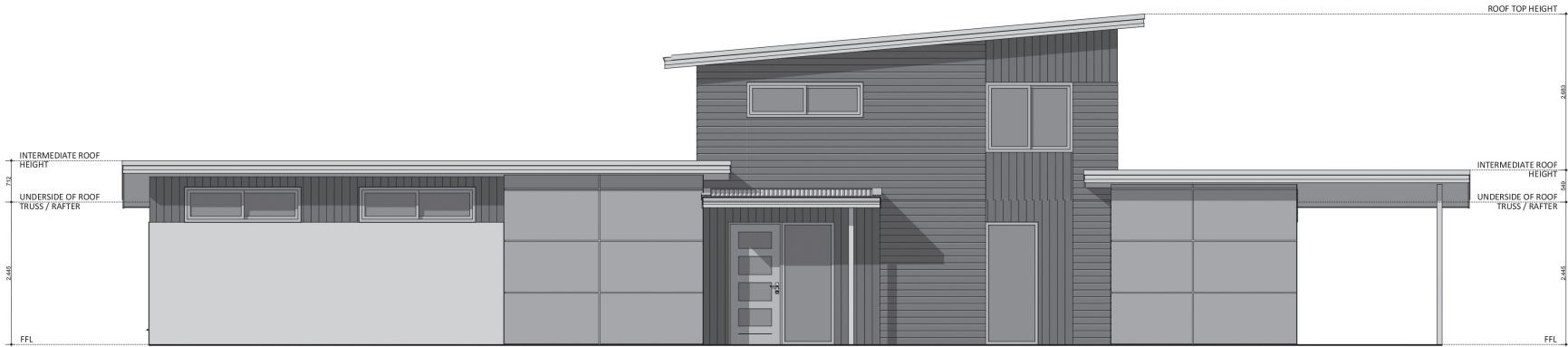
ELEVATION 03
