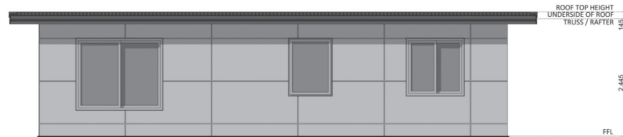
ELEVATION 03
