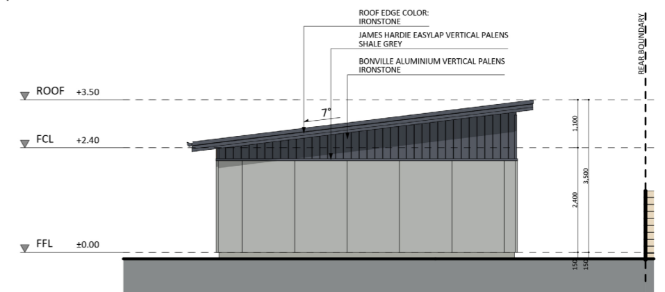
WEST ELEVATION
