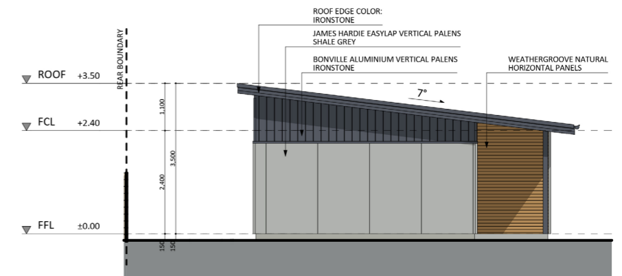
EAST ELEVATION
