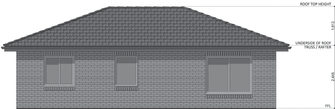
ELEVATION 03
