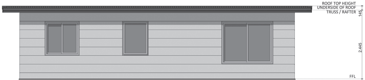
ELEVATION 03
