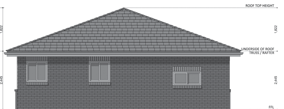
ELEVATION 03
