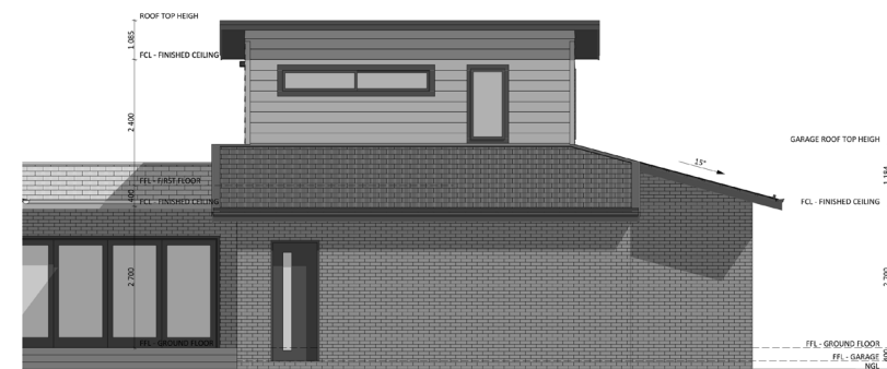
SOUTH-EAST ELEVATION
