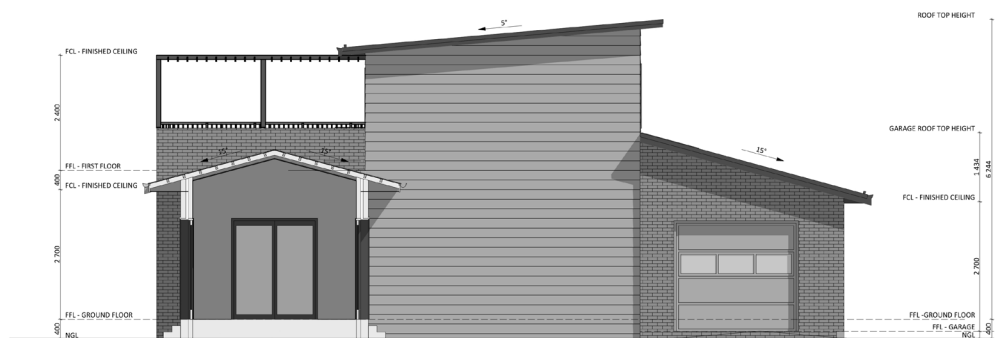
SOUTH-WEST ELEVATION
