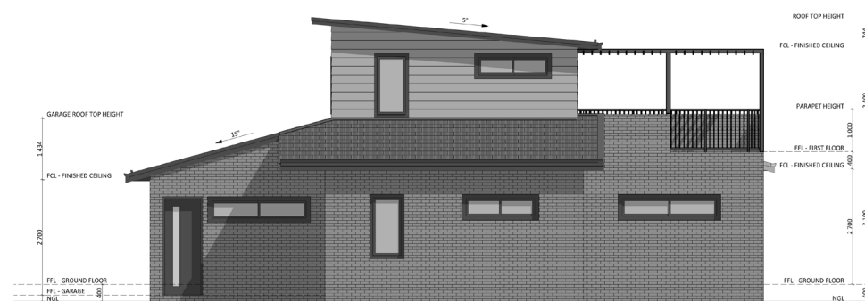
NORTH-EAST ELEVATION
