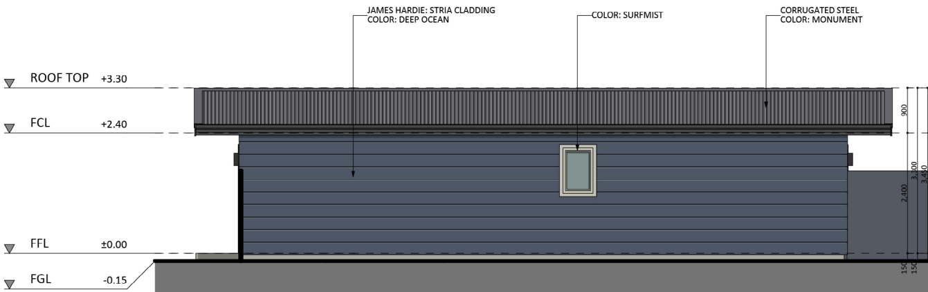
NORTH-EAST ELEVATION
