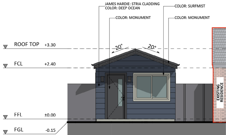
SOUTH-EAST ELEVATION
