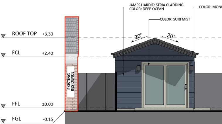
NORTH-WEST ELEVATION
