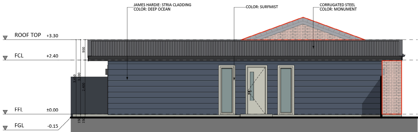
SOUTH-WEST ELEVATION
