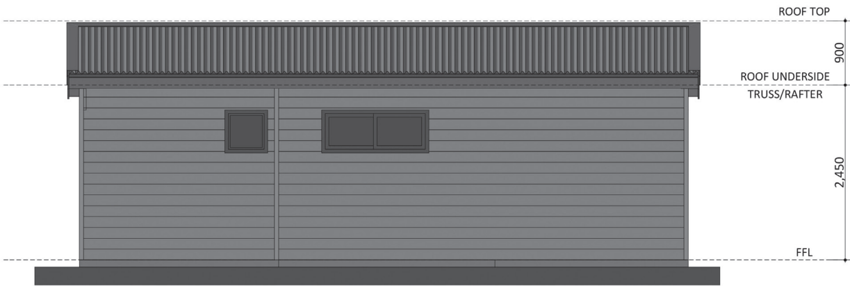
ELEVATION 03
