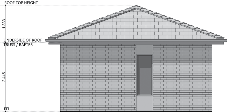
ELEVATION 03
