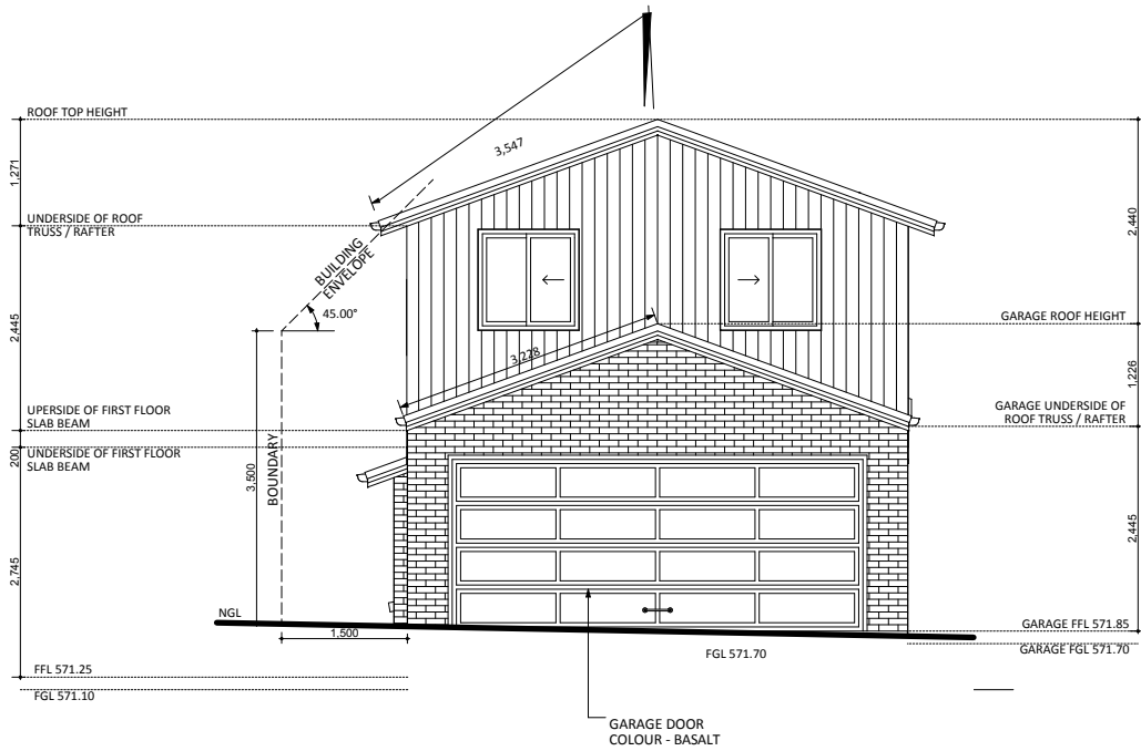
ELEVATION 03
