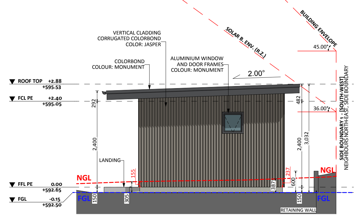
ELEVATION 03
