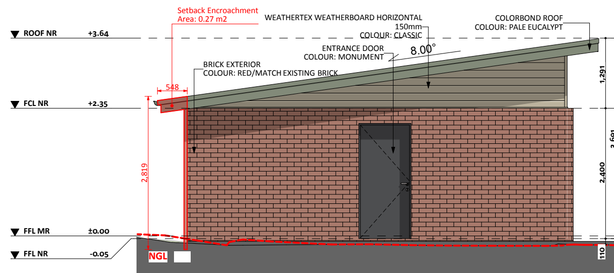
ELEVATION 03
