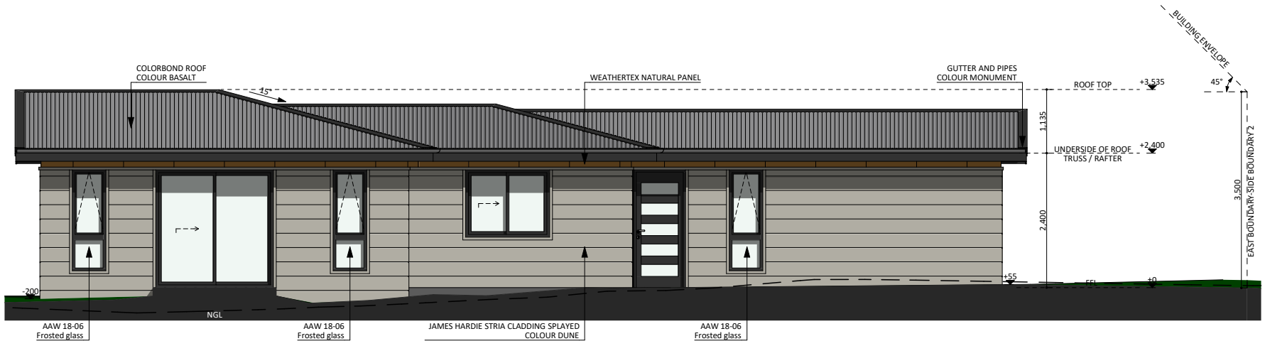
SOUTH ELEVATION
