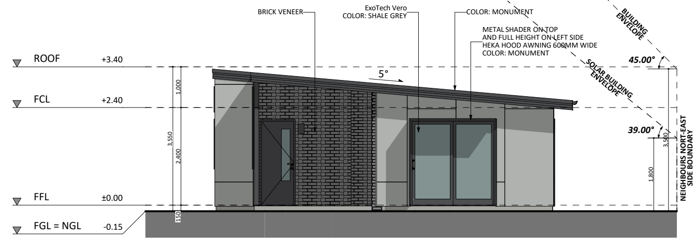
NORTH-WEST ELEVATION
