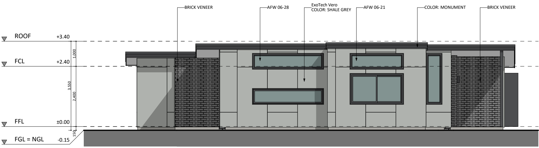
NORTH-EAST ELEVATION
