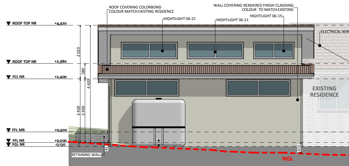
ELEVATION 03
