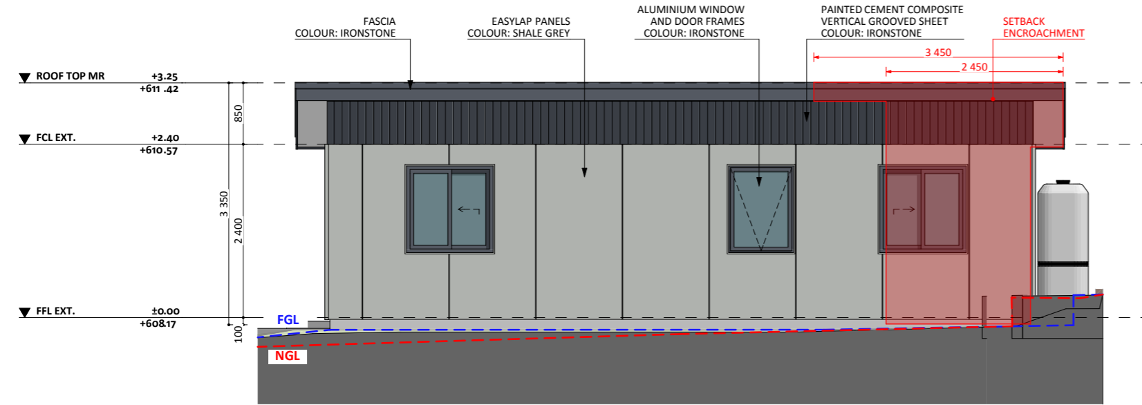
ELEVATION 03
