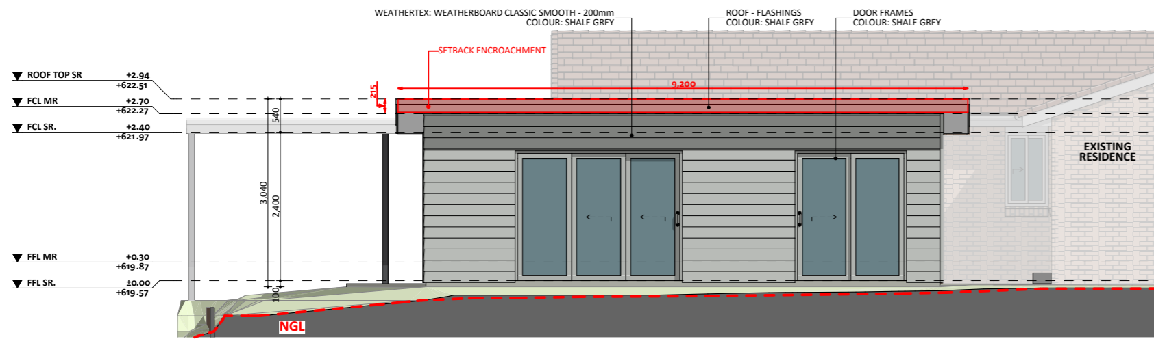
NORTH ELEVATION 01
