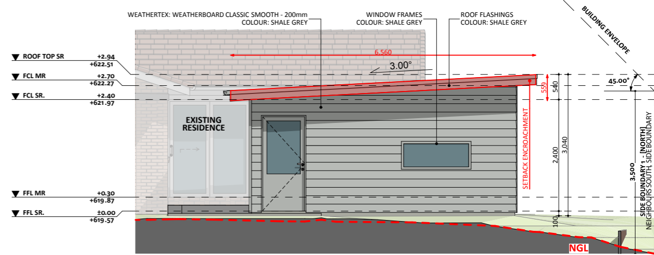
EAST ELEVATION 02
