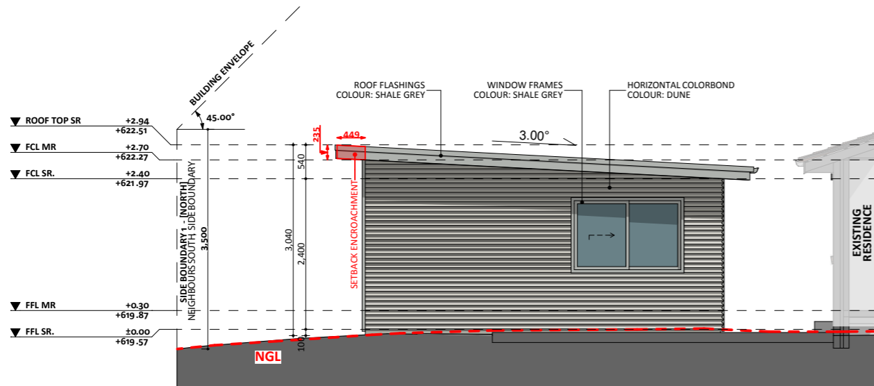
WEST ELEVATION 03
