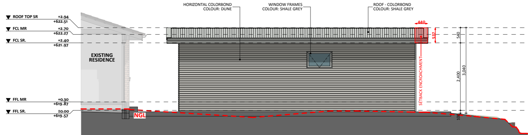
SOUTH ELEVATION 04
