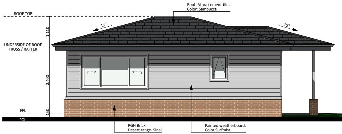
EAST ELEVATION
