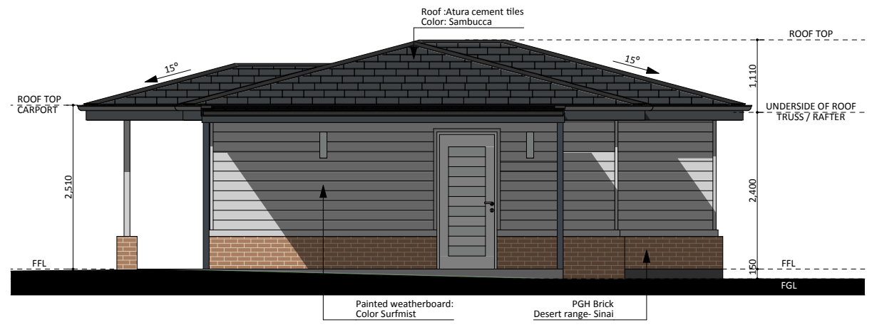
WEST ELEVATION
