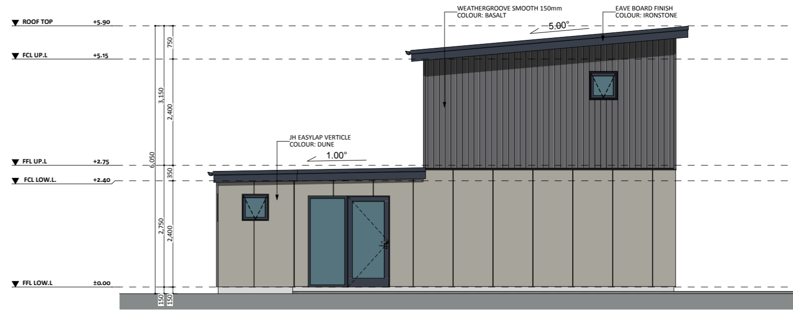
EAST ELEV.
