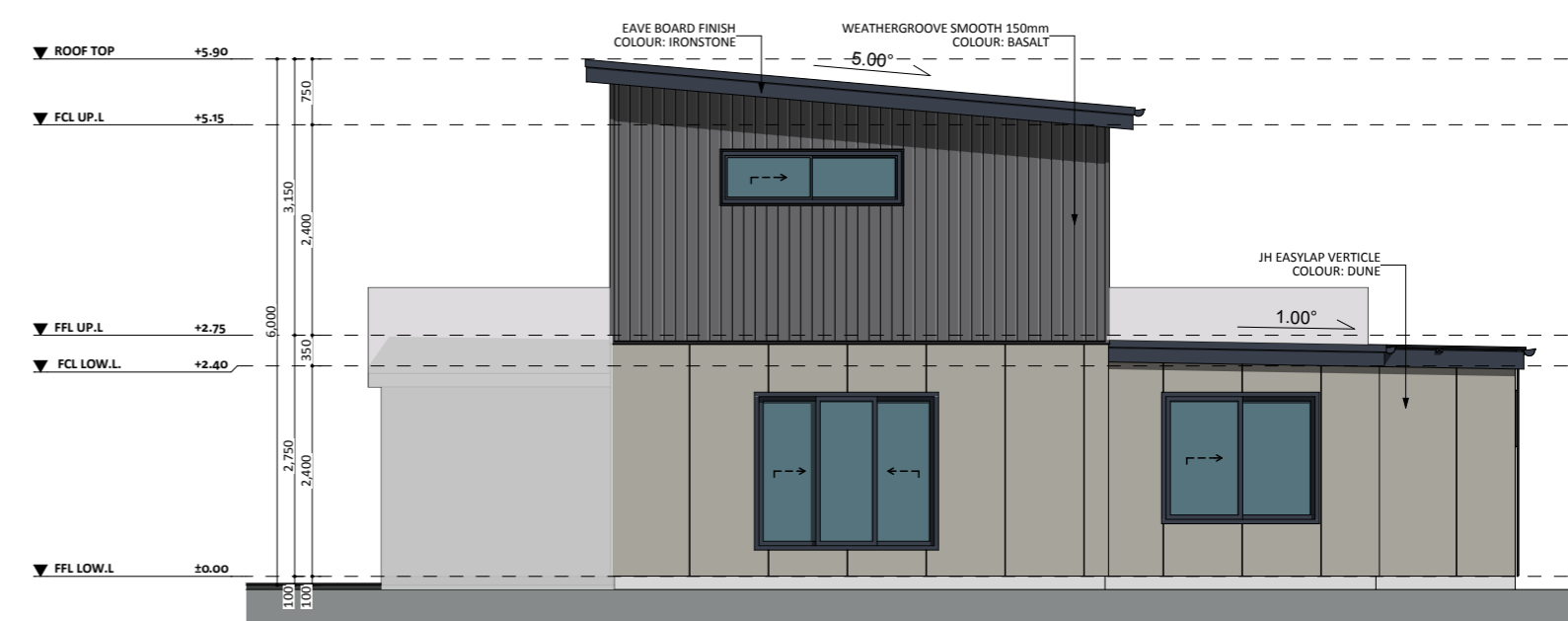
WEST ELEV.
