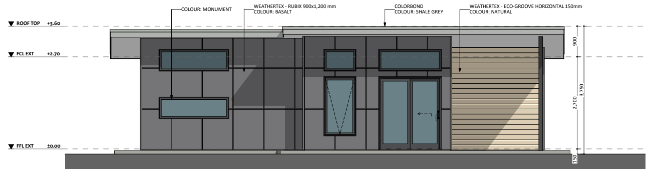
WEST ELEV.
