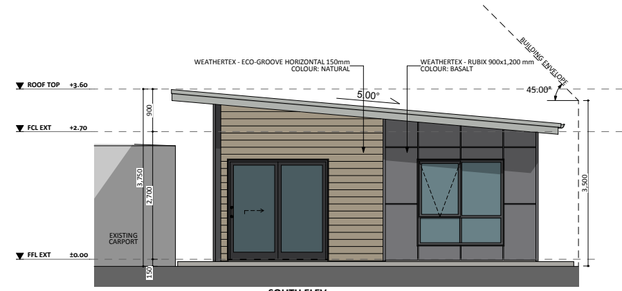
SOUTH ELEV.
