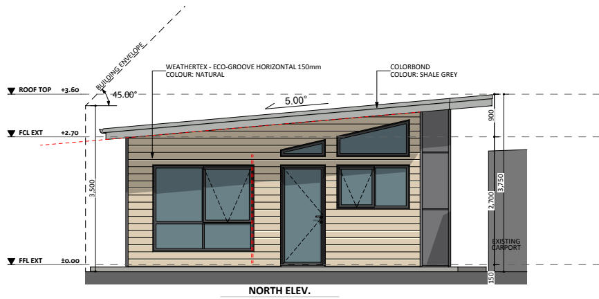
NORTH ELEV.
