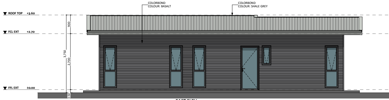
EAST ELEV.
