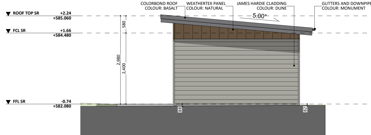
NORTH-EAST ELEV.
