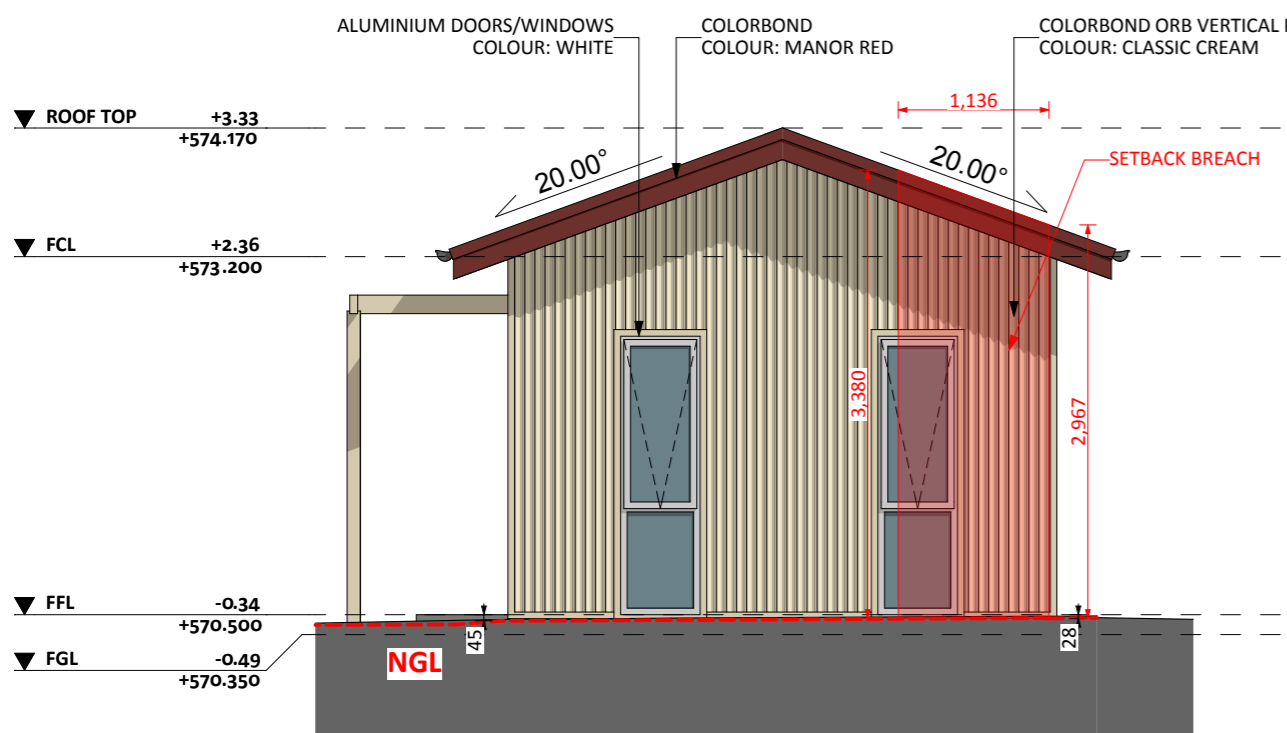
ELEVATION 03
