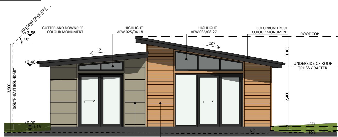
NORTH-EAST ELEVATION
