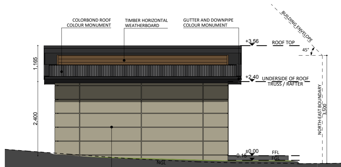
SOUTH-EAST ELEVATION
