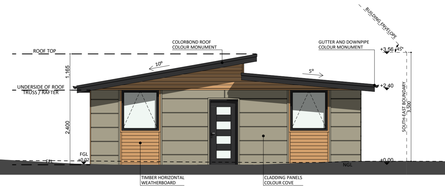
SOUTH-WEST ELEVATION
