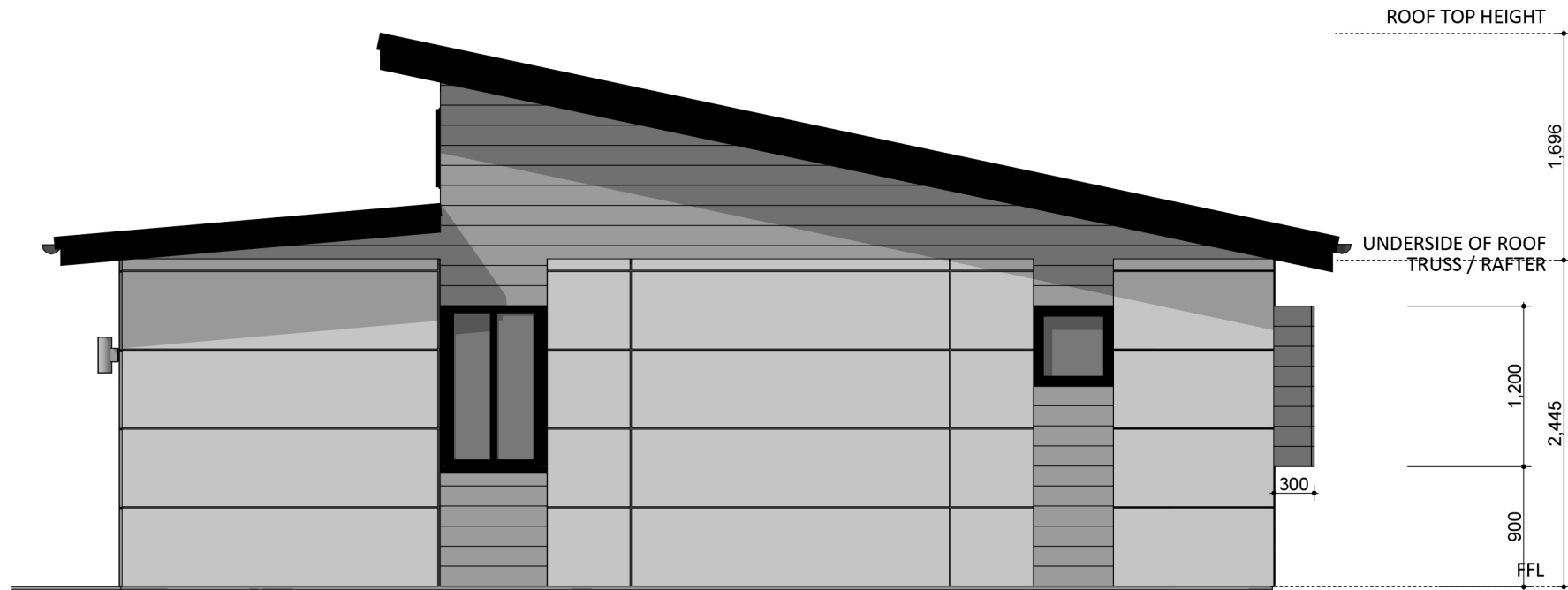
ELEVATION 03
