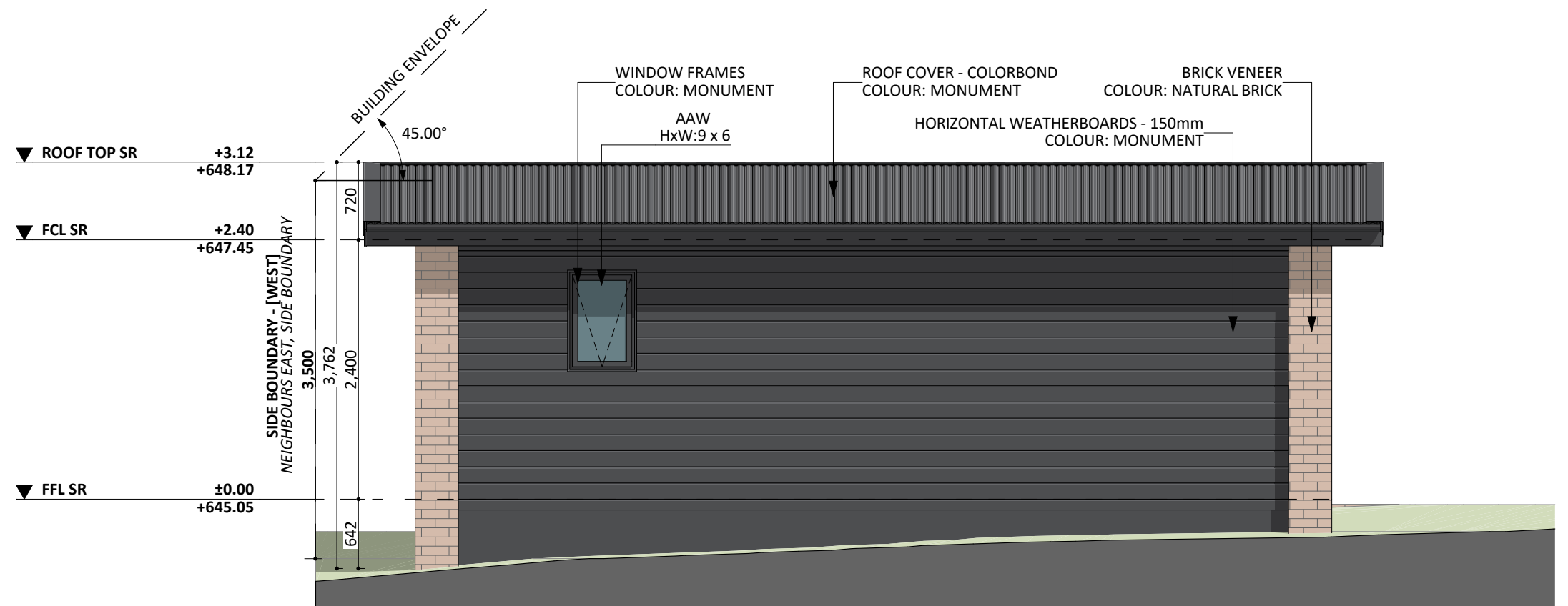
SOUTH ELEV.
