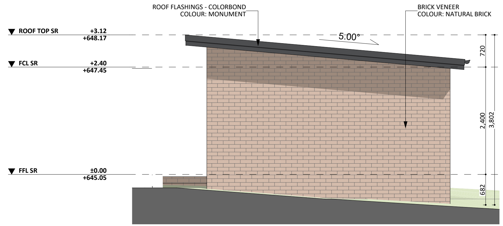
WEST ELEV.
