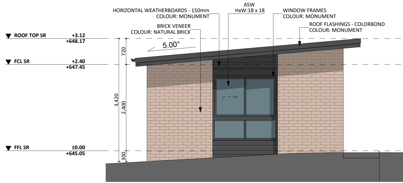
EAST ELEV.
